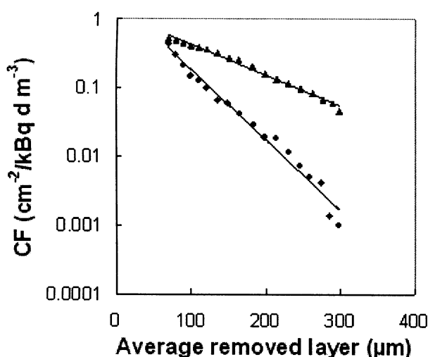
Fig. 2. Depth distribution of the response of CDs, represented by a calibration factor ( \text{CF} = \text{net-track density}/\text{integrated } ^{222}\text{Rn} \text{ concentration} ). Results at a temperature of 38°C ( \blacktriangle ) and 5°C ( \blacklozenge ).
