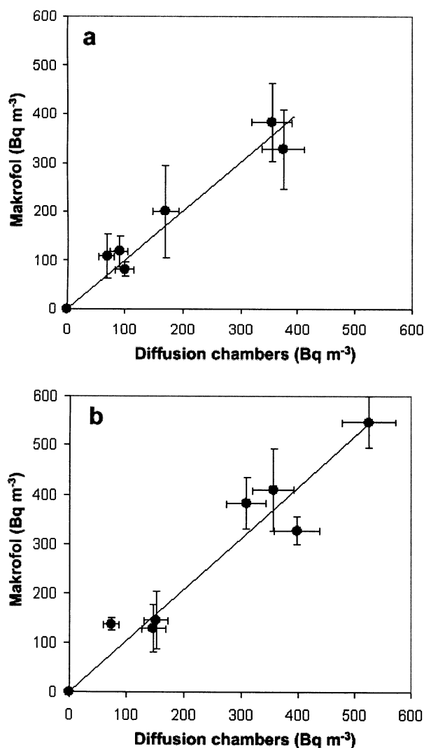
Fig. 3. Parallel measurements by polycarbonates (300 \mu\text{m} Makrofol foils) and diffusion chambers with Kodak-Pathe LR-115/II detectors. The exposure time was 301 days. Results are for (a) smoking rooms, and (b) non-smoking rooms.
