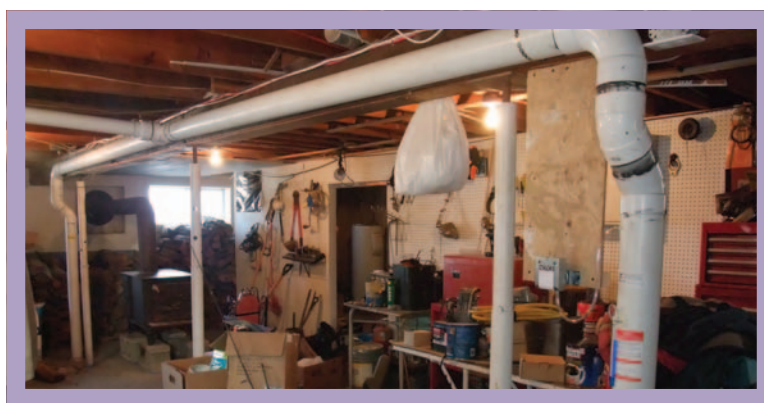
Photo 4 – Two Suction Point System
