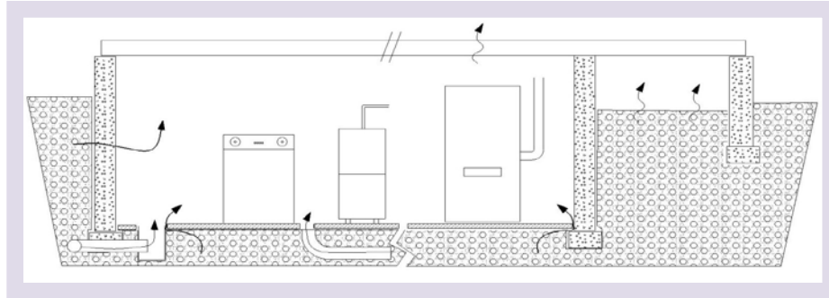
Figure 5 – Radon Entry Routes for a Poured Concrete Foundation
