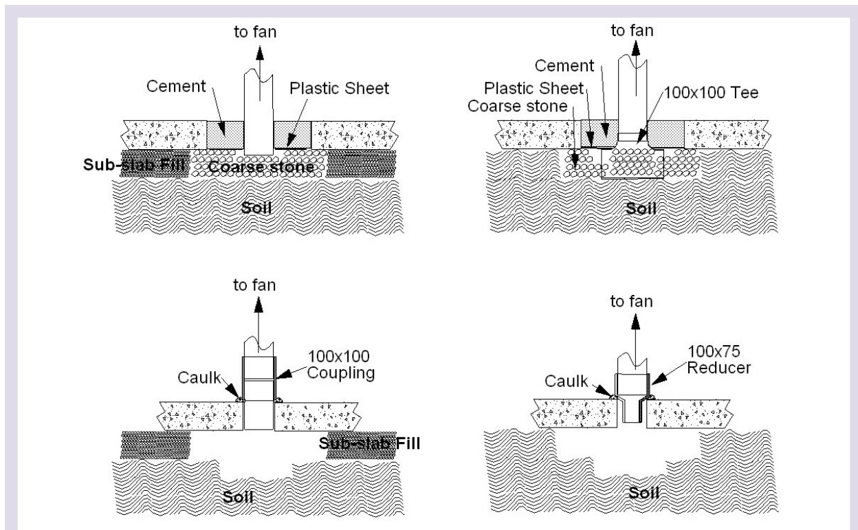
Figure 9 – Exhaust Pipe Connection Details
