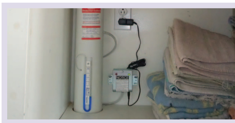
Photo 11 - Two devices used to insure the functionality of the soil depressurization system: a pitot tube and an audible alarm
