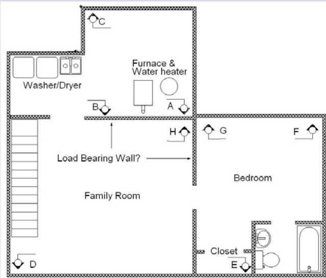
Figure 8 - Test Hole Layout Example
