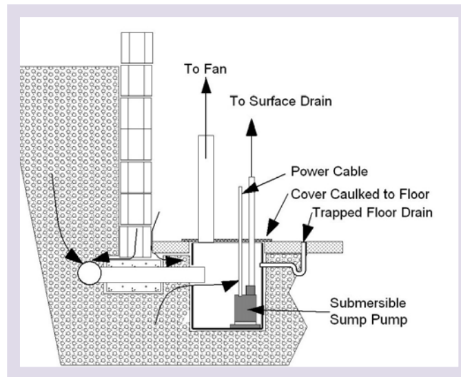
Figure 12 – Sump Exhaust
