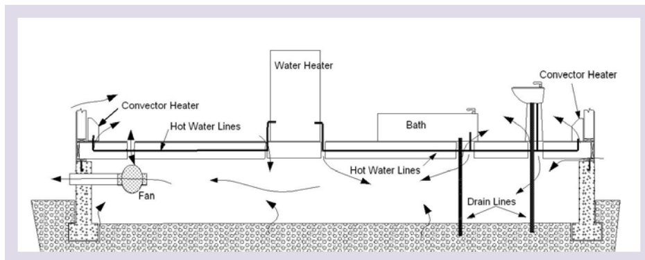
Figure 14 – Crawlspace Exhaust
