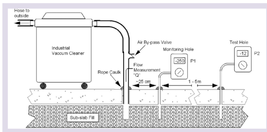
Figure 7 – Sub-Slab Communication Test
