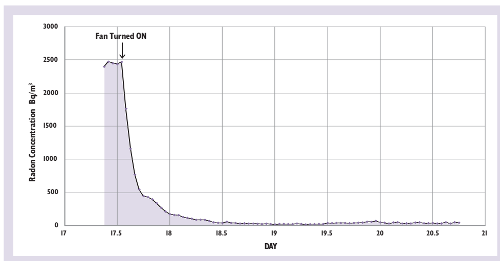
Figure 15 – Change in Radon Concentration after Mitigation
