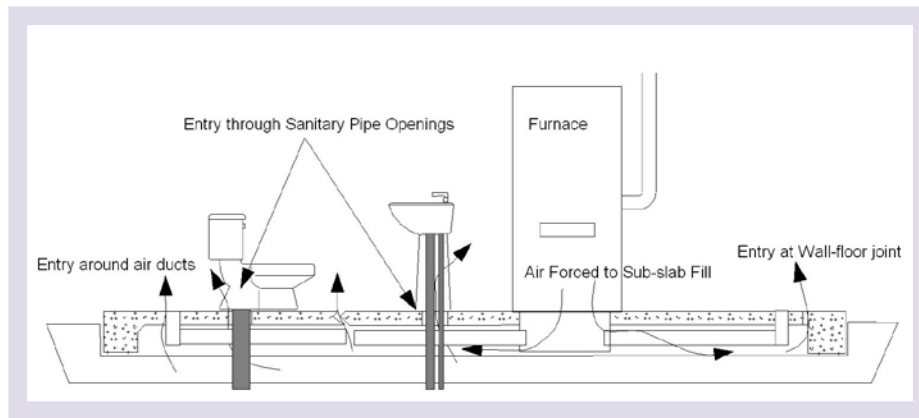
Figure 6 – Radon Entry Routes for a Slab on Grade Foundation
