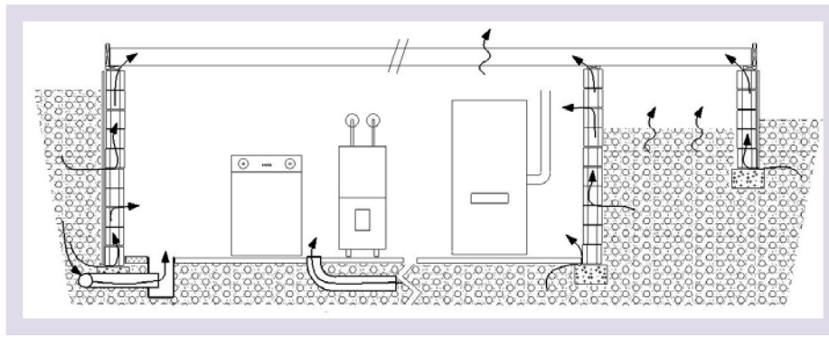
Figure 4 – Radon Entry Routes for a Hollow Concrete Block Foundation
