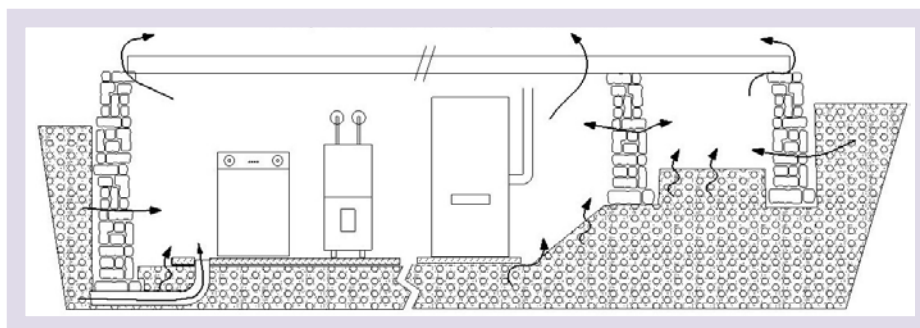
Figure 3 - Radon Entry Routes for a Masonry Basement or Cellar Foundation
