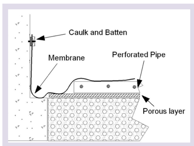
Figure 11 – Membrane and Wall Attachment
