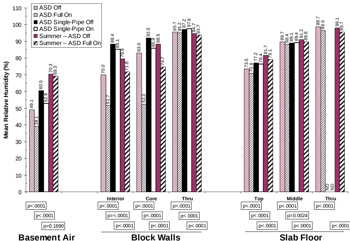
Figure 21. Arithmetic mean RH for second 7 days of 14-day, or longer, cycling periods at PA03. These data are for December 2005 through January 2007, and include summer periods, and periods when the ASD operation was reduced to a single sub-slab pipe. When data were not available, it is indicated by ND.
