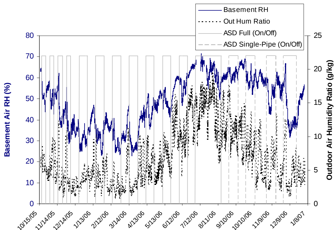
Figure 10. Moisture levels in basement air (RH) and outdoor air (humidity ratio, W) over a 15-month period at PA02, during ASD system cycling.
