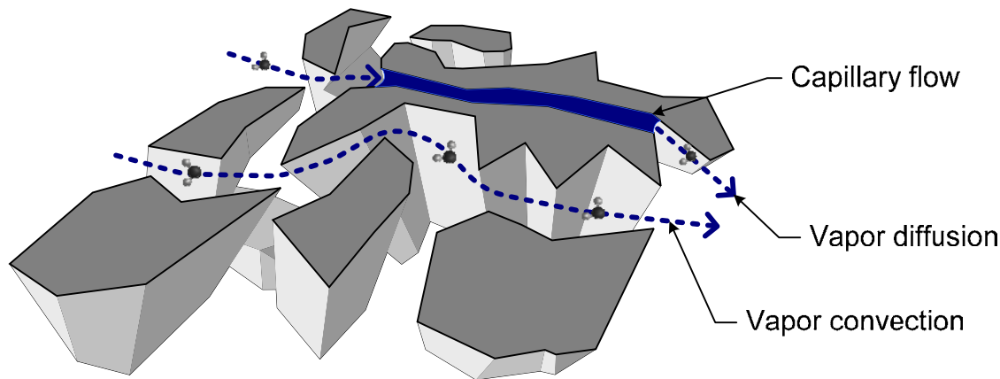
Figure 3: Capillary, diffusive, and convective moisture flows in a porous material
